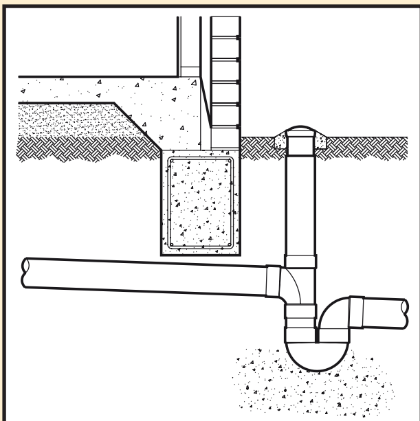
Typical ORC device installation
