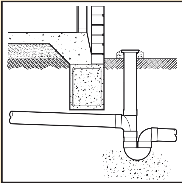
Conventional ORG installation
