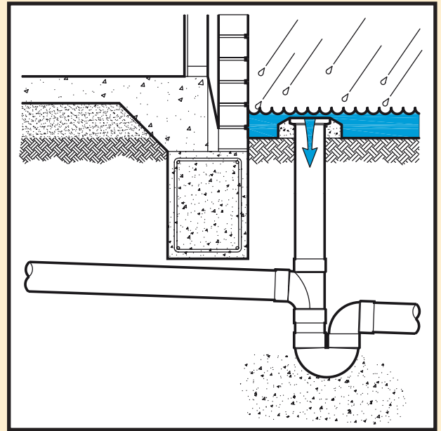
ORG allowing water ingress
