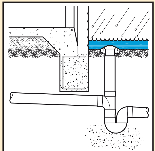
ORC device sealing against water ingress
