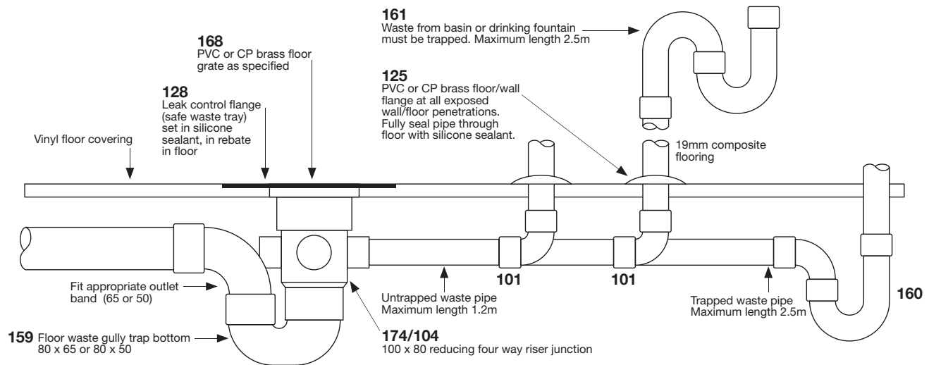
Figure 20 - Typical Floor Waste Gully Design & Installation Requirements
