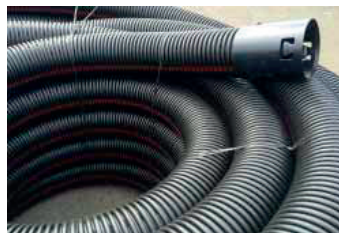
Iplex NEXUS HI-WAY pipe coil showing the pull-out resistant coupling and red stripe for visual identification
