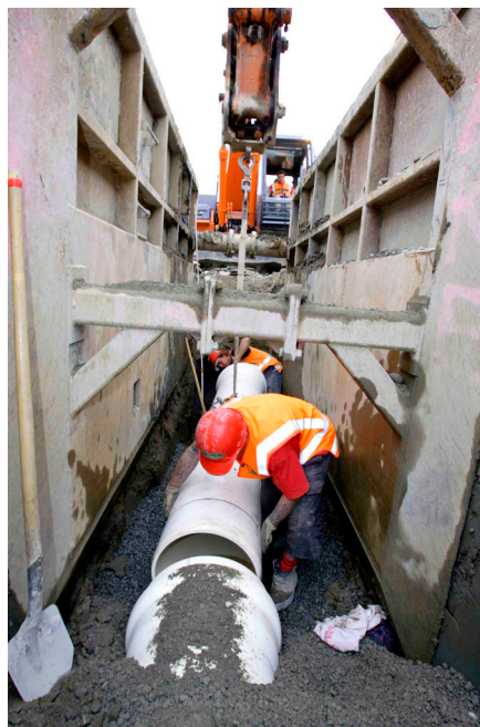
Installation of Iplex PVC pressure sewer rising main, Belfast, Christchurch City.
