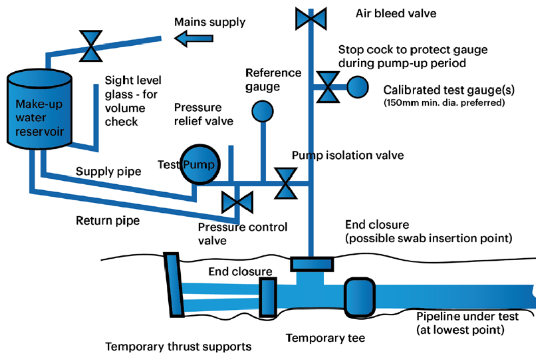
Figure 6.31 - Typical arrangement of pressure test equipment
