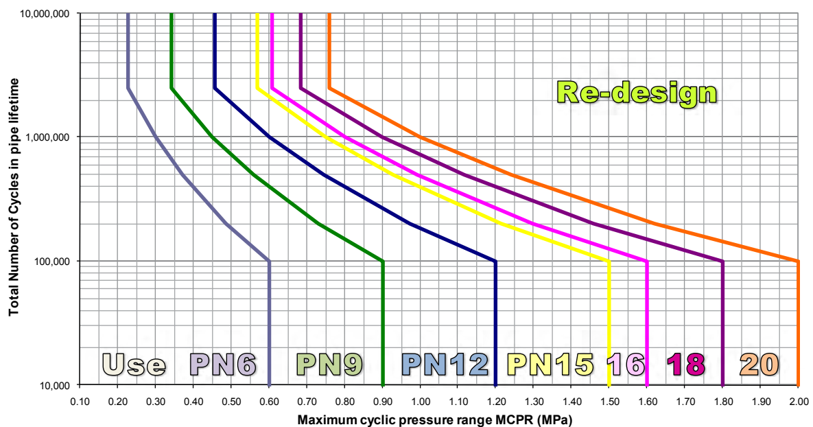
Figure 4.7 Selection of PVC-U Pressure Class Fatigue Applications
