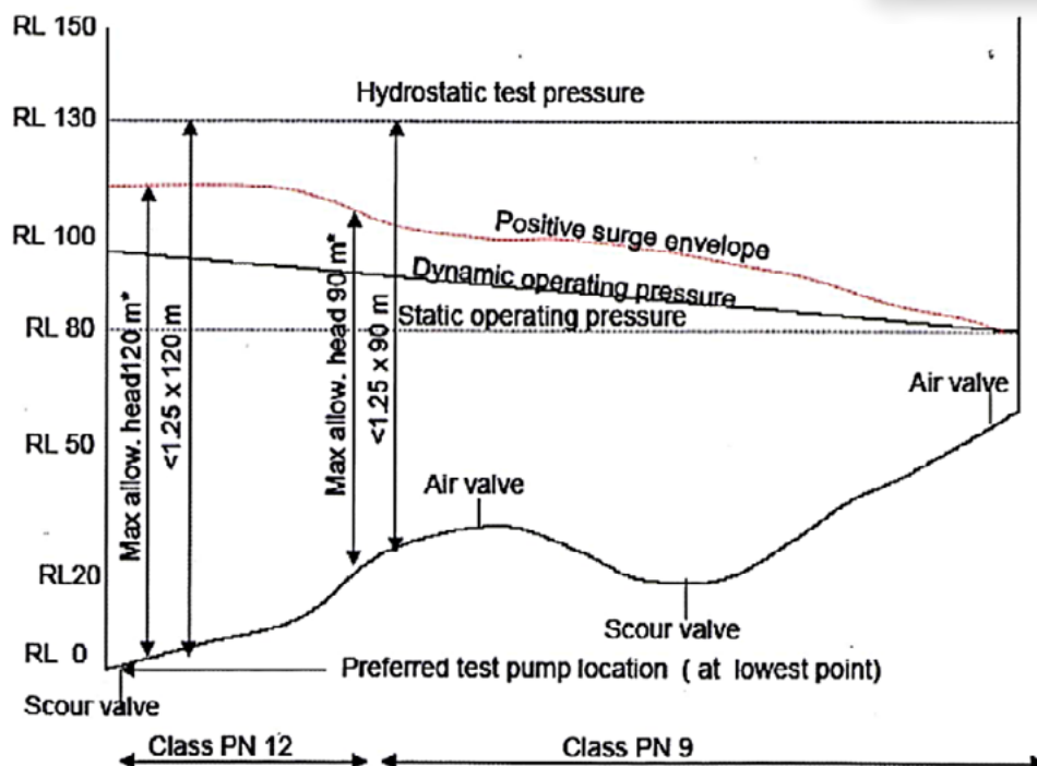
Figure 6.30 - Longitudinal section of pipeline for determining appropriate hydrostatic test pressures
