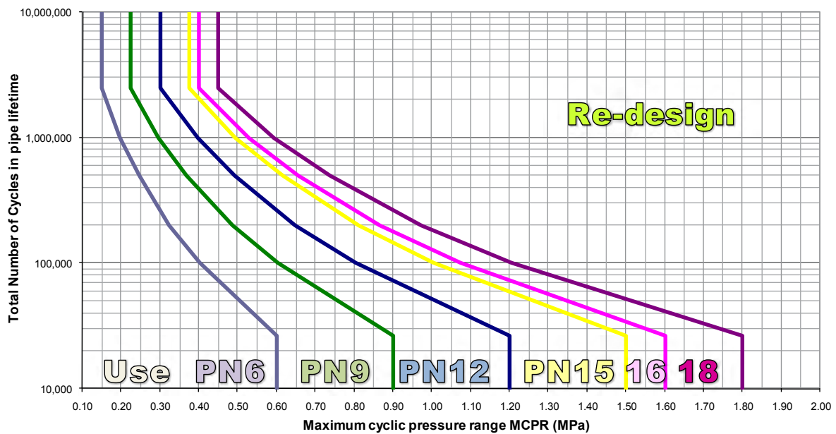
Figure 4.6 Selection of PVC-M Pressure Class Fatigue Applications
