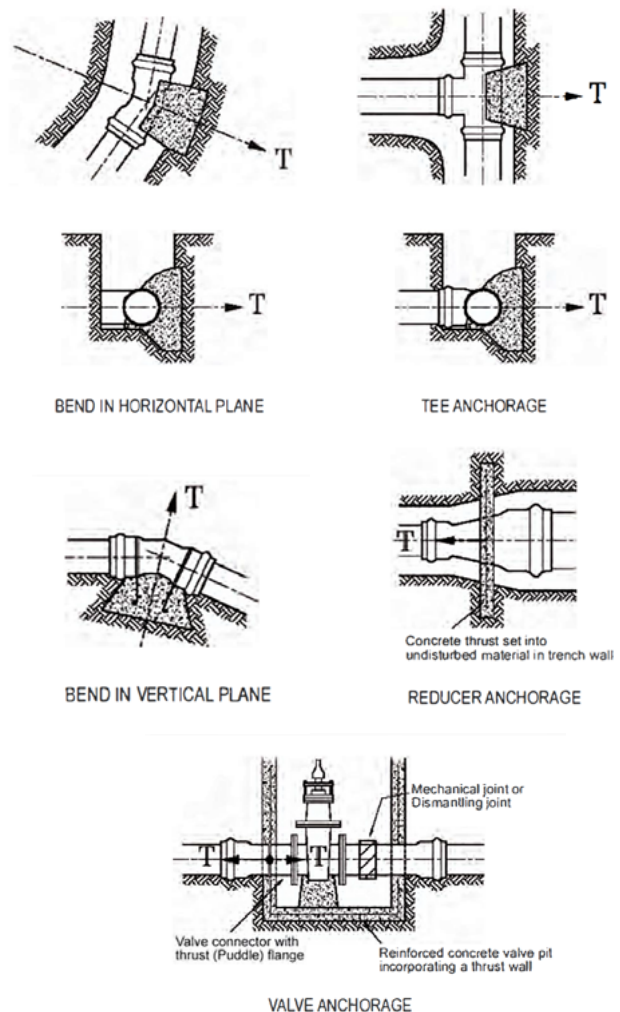
Figure 5.6 - Typical thrust block arrangements (Reference: AS / NZS 2566)
