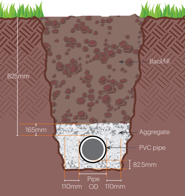
Fig. 1 Typical Open Cut Trench Installation
