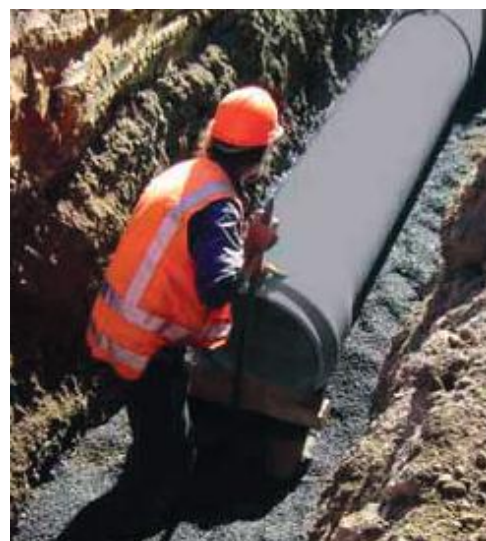
Figure 18 - Push joint home until witness mark remains just visible
