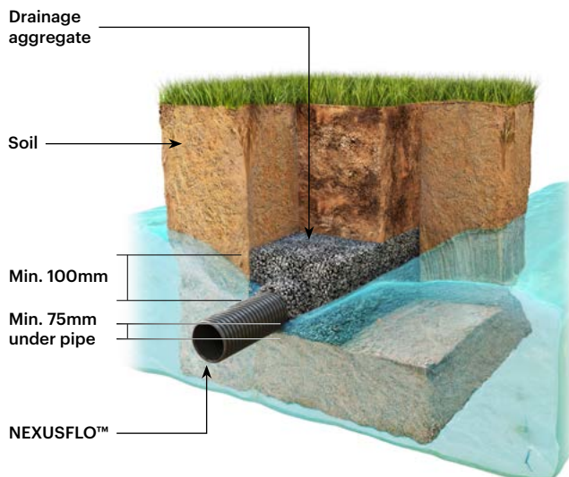
Standard installation in permeable non-sandy soils - NEXUSFLO™ encased in drainage aggregate envelope designed as a filter
