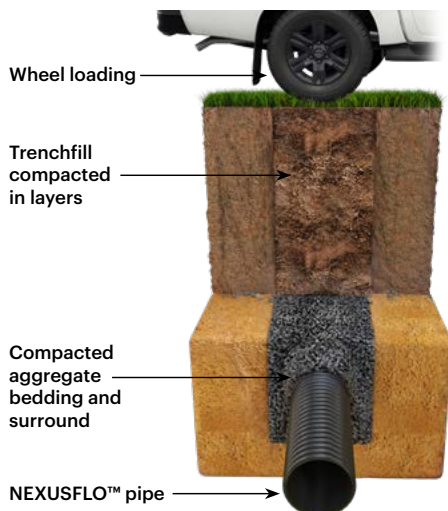
NEXUSFLO™ crossing a farm raceway with thoroughly compacted aggregate surround and backfill
