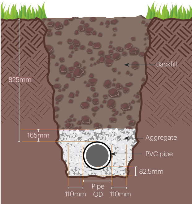
Fig. 1 Typical Open Cut Trench Installation
