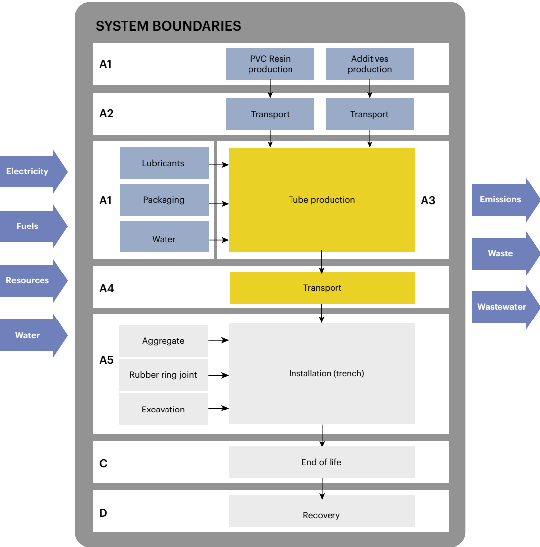
Fig. 2 System boundaries diagram
