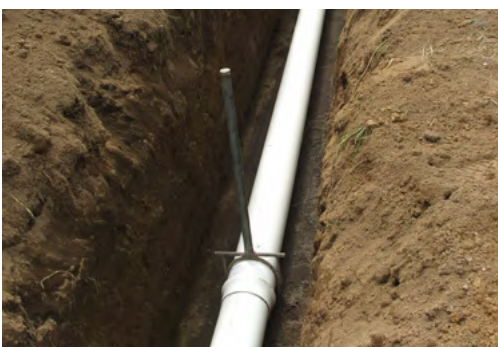
Figure 6.19 - Positioning of pipe jointing fork
