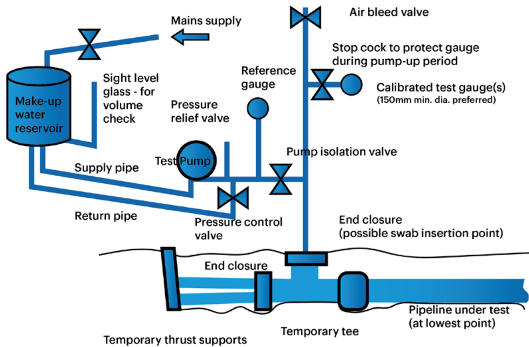
Figure 6.31 - Typical arrangement of pressure test equipment
