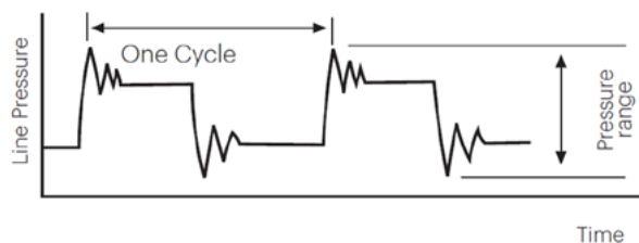
Figure 4.4 Pressure Cycle
