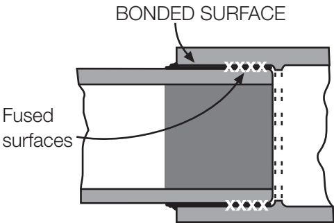
Fused and bonded surfaces of joined pipe and fitting
